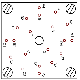
PIN LOCATIONS DESIGNATION FOR REFERENCE ONLY. (CONTACT PANEL IS NOT MARKED).
