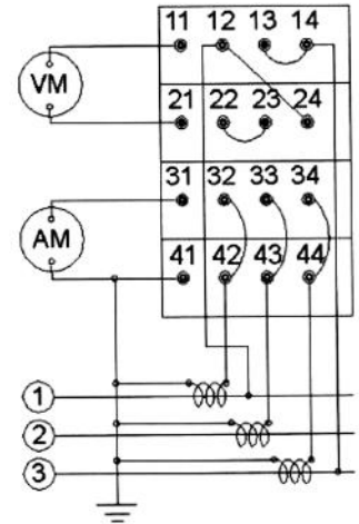
WIRING DIAGRAM
