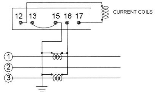
WIRING DIAGRAM
