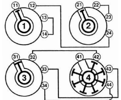
Deck 3 & 4 make-before-break contacts
