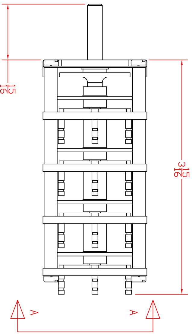
VIEW A - A
