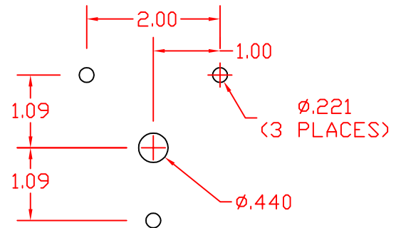
MOUNTING HOLE DETAIL
