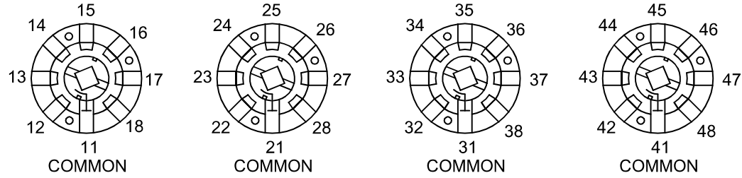
SCHEMATIC DIAGRAM
